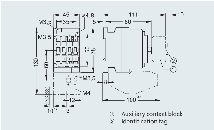
3TF32/33 AC Coil
