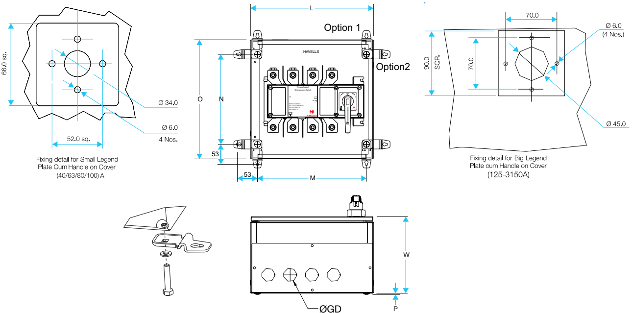
Dimension (in mm) - Enclosure
