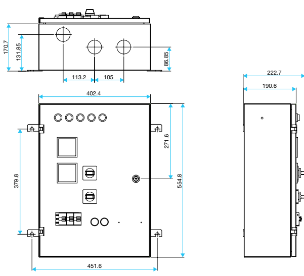
ASD Submersible Pump Starter 27.5HP - 45HP (Deluxe)
