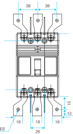
Three Pole with Extended Terminals
