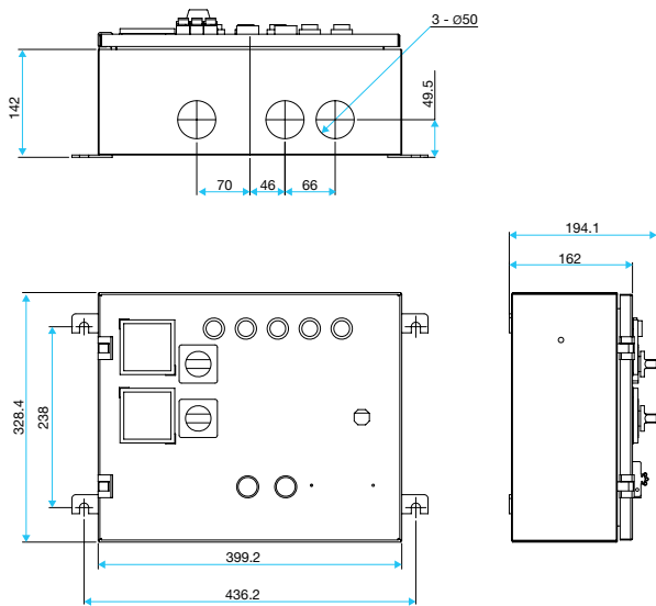
ASD Submersible Pump Starter 5HP - 25HP (Standard)
