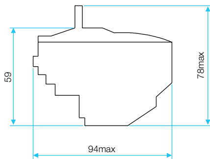
Without adapter block
