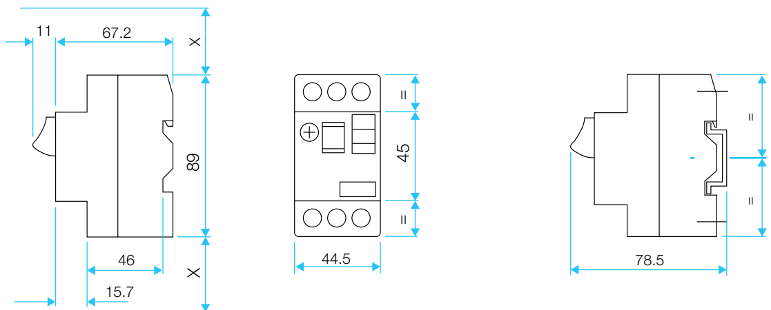
Dimension (in mm)
