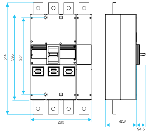
Four Pole with Switched Neutral
