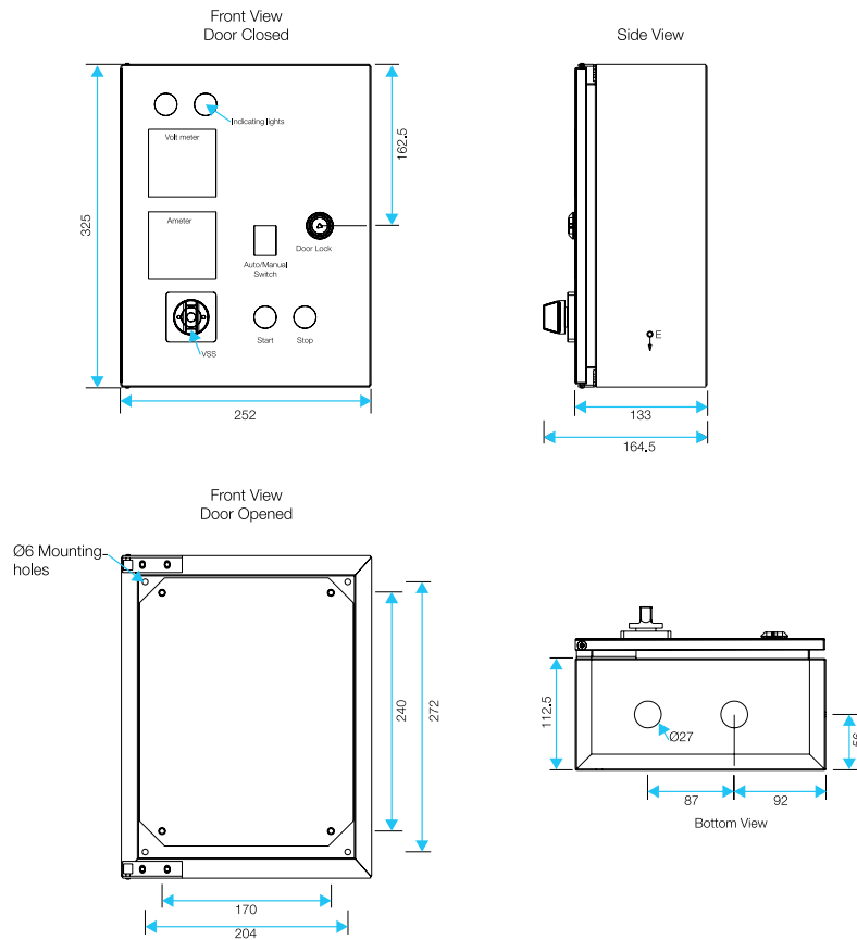
Dimensional Drawing DOL (Size in mm)
