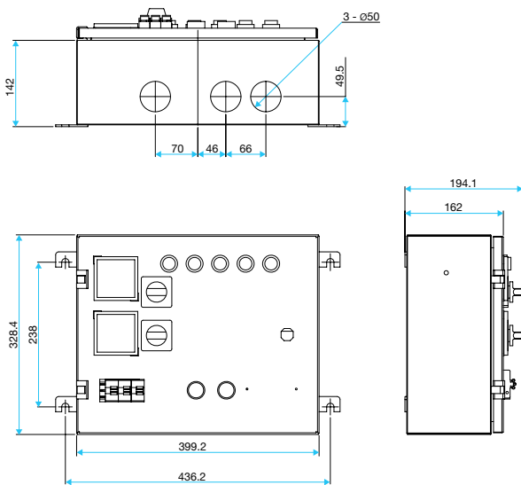
ASD Submersible Pump Starter 5HP - 25HP (Deluxe)
