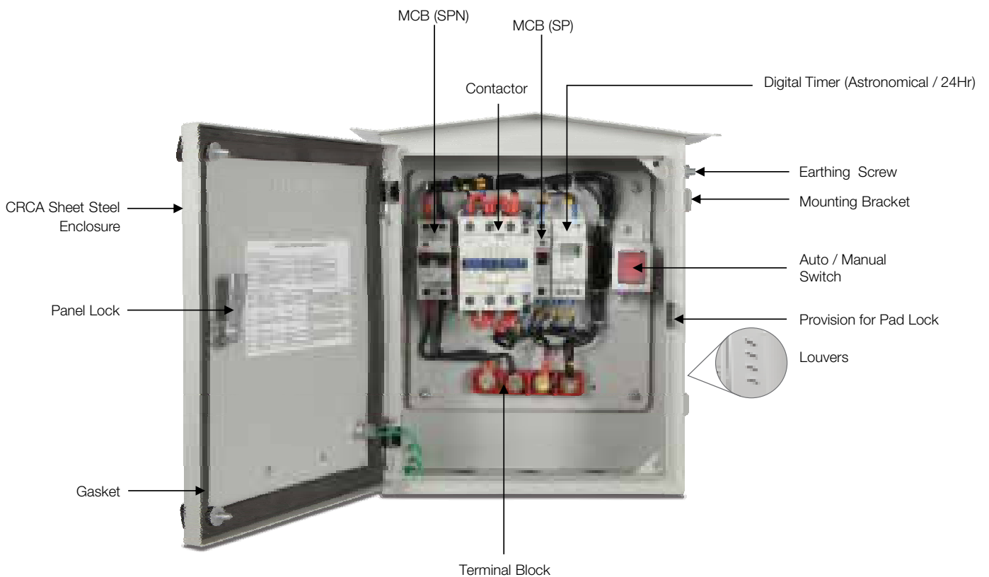
Single Phase Street Light Panel with 24Hrs / Astronomical Timer
