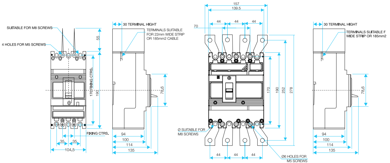
Three Pole
