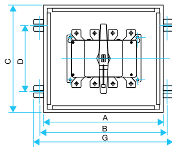
1000A to 3150A
