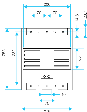
Three Pole
