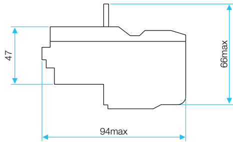
Without adapter block
