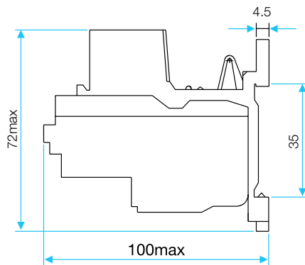
With adapter block
