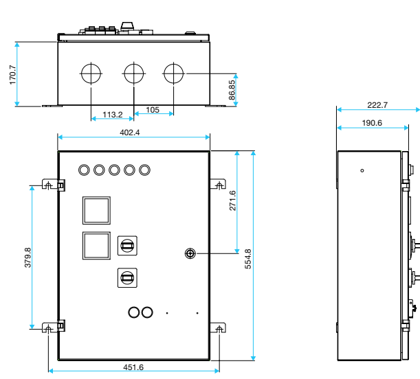
ASD Submersible Pump Starter 27.5HP - 45HP (Standard)
