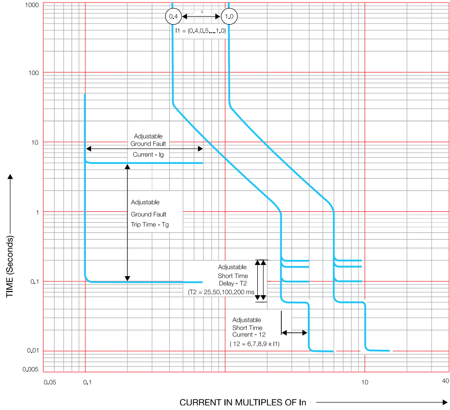
Ground Fault & Over Current Tripping Characteristics
