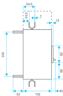
Three Pole
