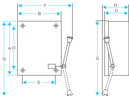
Fabricated Enclosure
