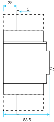
Three Pole with Extended Terminals
