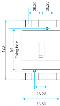
Three Pole
