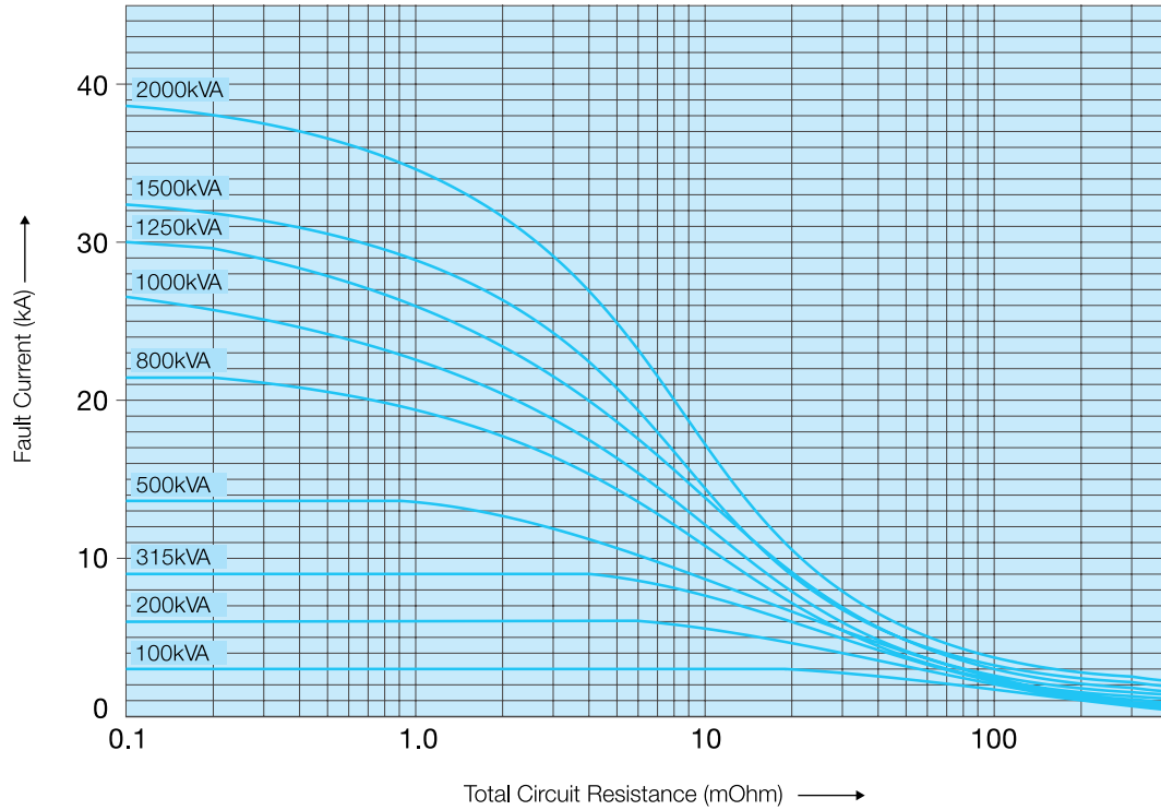
Estimating the Prospective Short Current
